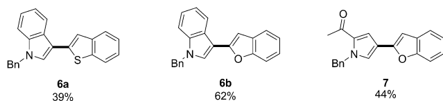
Figure 1. Coupling products and yields of isolated products for the reactions of N -benzylindole and N -benzyl-2-acetylpyrrole with benzofuran and/or benzothiophene. [34]
